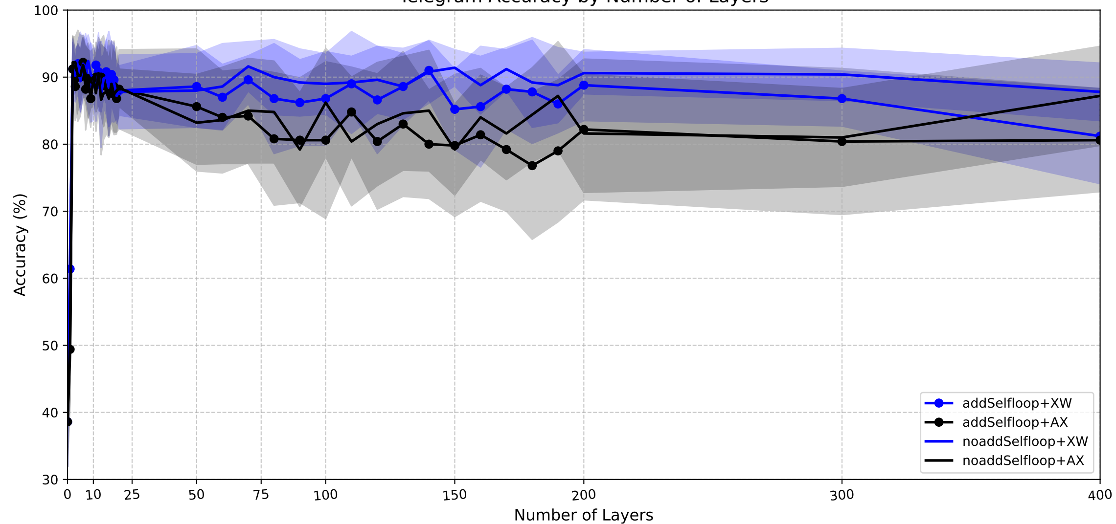
Telegram Accuracy by Number of Layers
